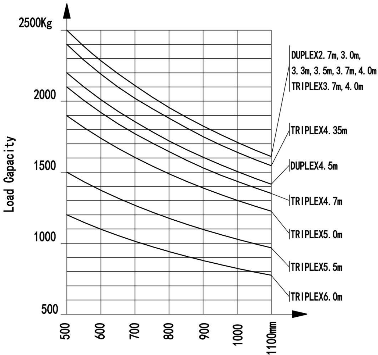
2.5T Rough Terrain Forklift Load Curve
