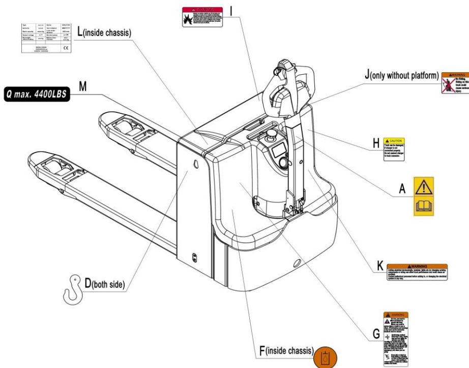
Fig. 26: Warning labels and safety devices PT 20L-Li (only USA)
