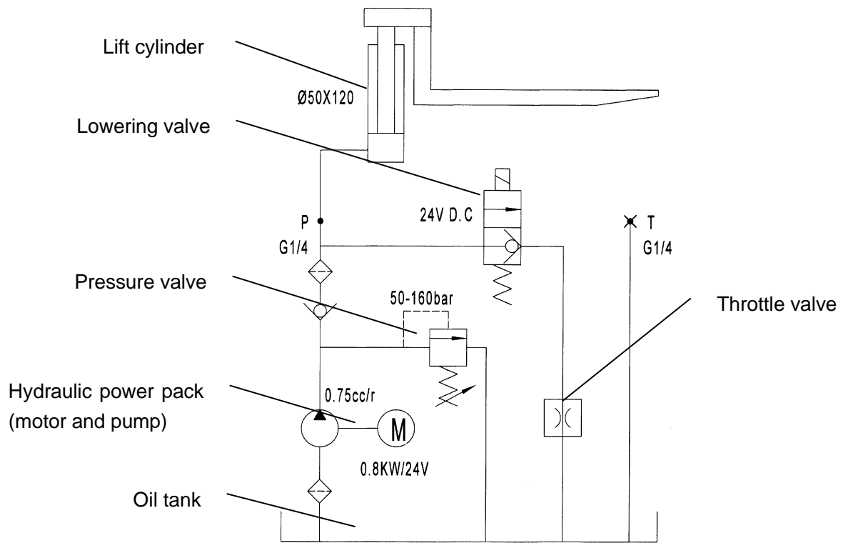
Fig.24: PT16L-Li&20L-Li Hydraulic circuit
