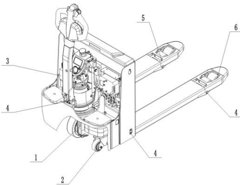
Fig. 18: Lubricating points
