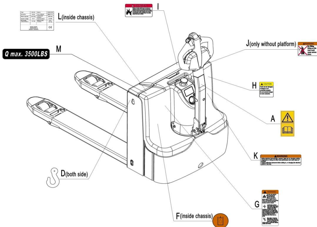
Fig. 25: Warning labels and safety devices PT 16L-Li (only USA)
