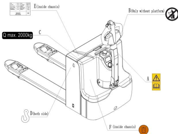
Fig. 5: Safety and warning labels PT 20L-Li
