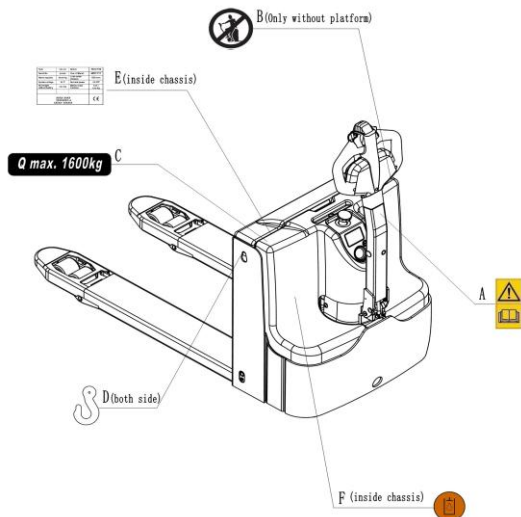
Fig. 4: Safety and warning labels PT 16L-Li
