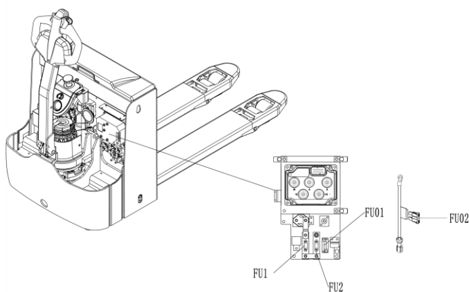
Fig. 19: Location fuses (PT16L-Li&20L-Li)
