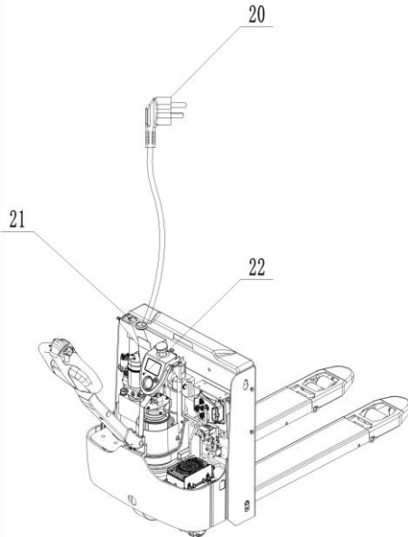
Fig.17: Battery Charging (Built-in Charger)
