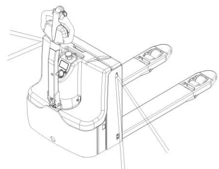
Fig. 8: fixing points
