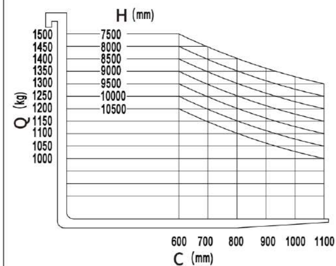
RT20SP10500E(Battery Capacity:900AH)
