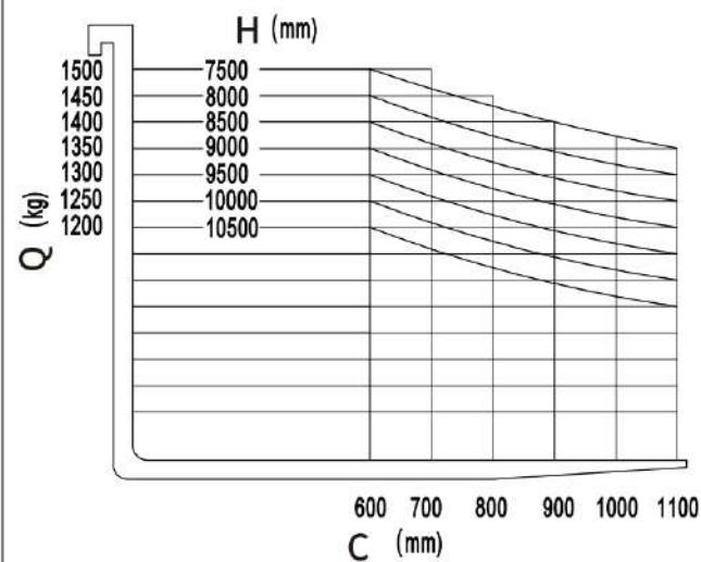
RT15DP10500E(Battery Capacity:900AH)
