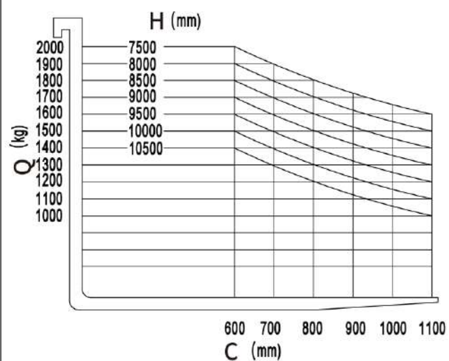
RT15SP10500D(Battery Capacity:800AH)
